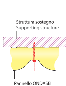
Montaggio verticale Vertical mounting
